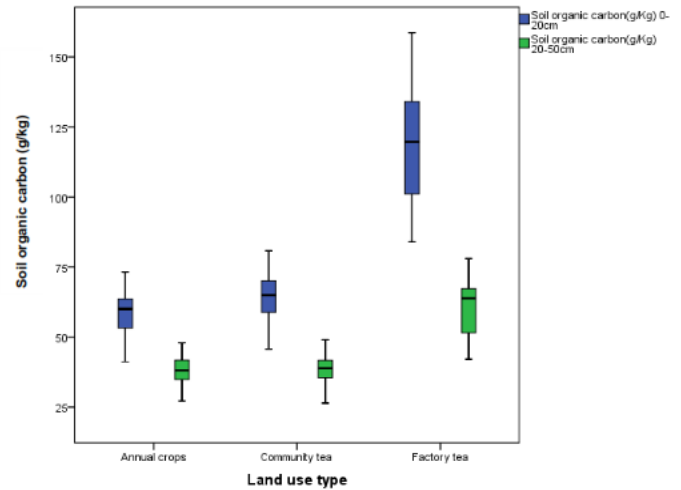
Figure 2: Soil organic carbon comparisons in annual crops, community tea and factory tea
