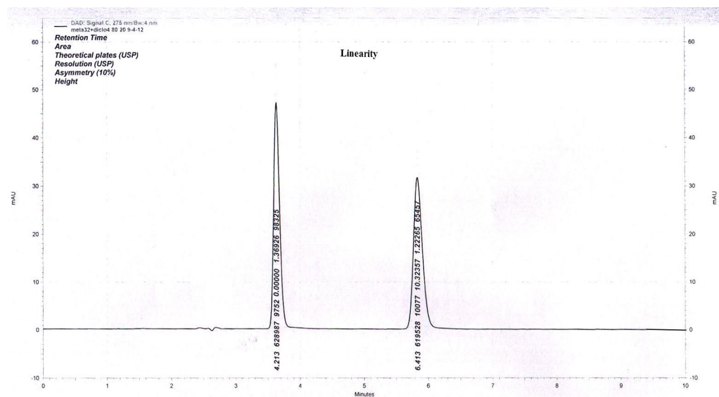
Figure 3: Optimized chromatogram for Levonorgestrel and Ethinylestradiol
