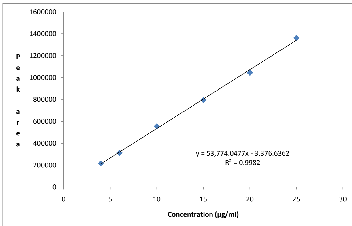
Figure 6: Linearity plot of Ethinylestradiol
