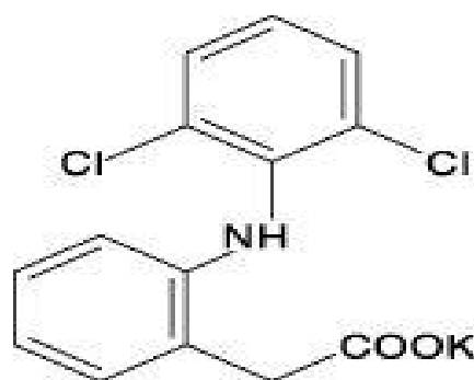
Figure 2: Structure of Ethinylestradiol potassium
