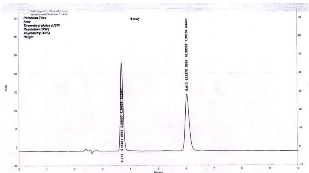
Figure 4: Assay chromatogram of Levonorgestrel and Ethinylestradiol
