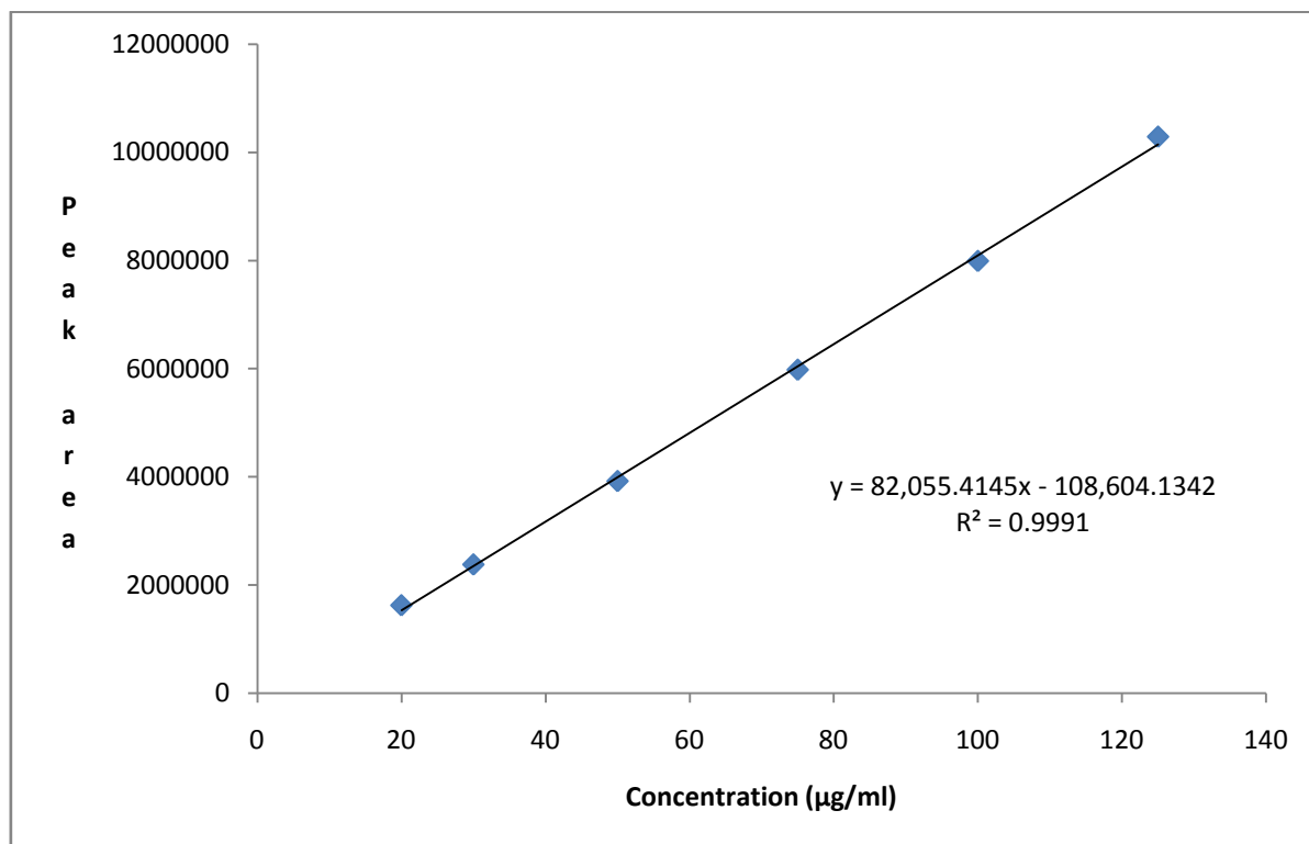
Figure 5: Linearity plot of Levonorgestrel
